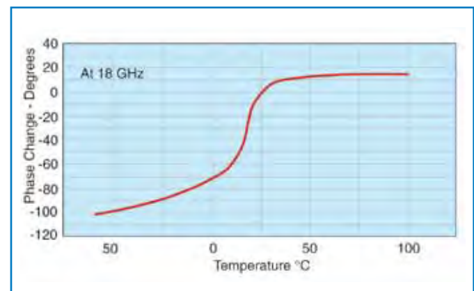
Fig. 10 Phase Stability
