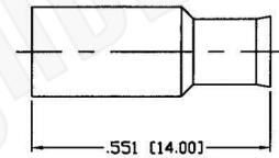
RECOMMENDED CRIMP DIE: .130" & .178"
