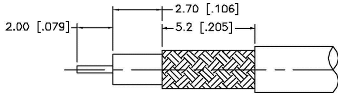
RECOMMENDED CABLE STRIPPING DIMENSIONS
