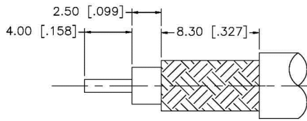
RECOMMENDED CABLE STRIPPING DIMENSIONS
