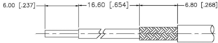
RECOMMENDED CABLE STRIPPING DIM'S
