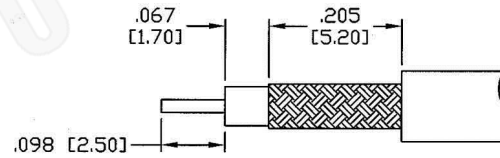
RECOMMENDED STRIPPING DIM'S
