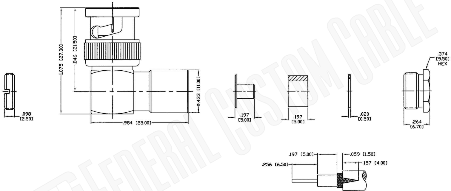
RECOMMENDED STRIPPING DIMENSIONS
