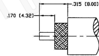
RECOMMENDED STRIPPING DIMENSIONS
