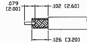
RECOMMENDED STRIPPING DIMENSIONS
