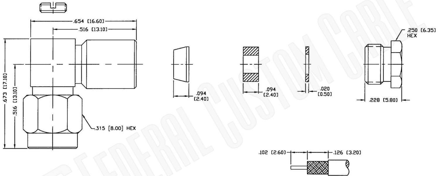
RECOMMENDED STRIPPING DIMENSIONS
