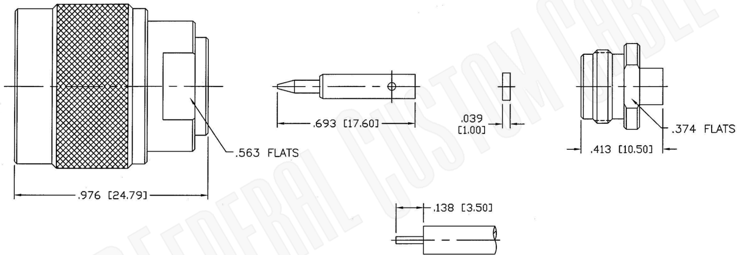
RECOMMENDED STRIPPING DIMENSIONS
