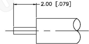
RECOMMENDED CABLE STRIPPING DIMENSIONS
