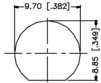
RECOMMENDED MOUNTING HOLE
