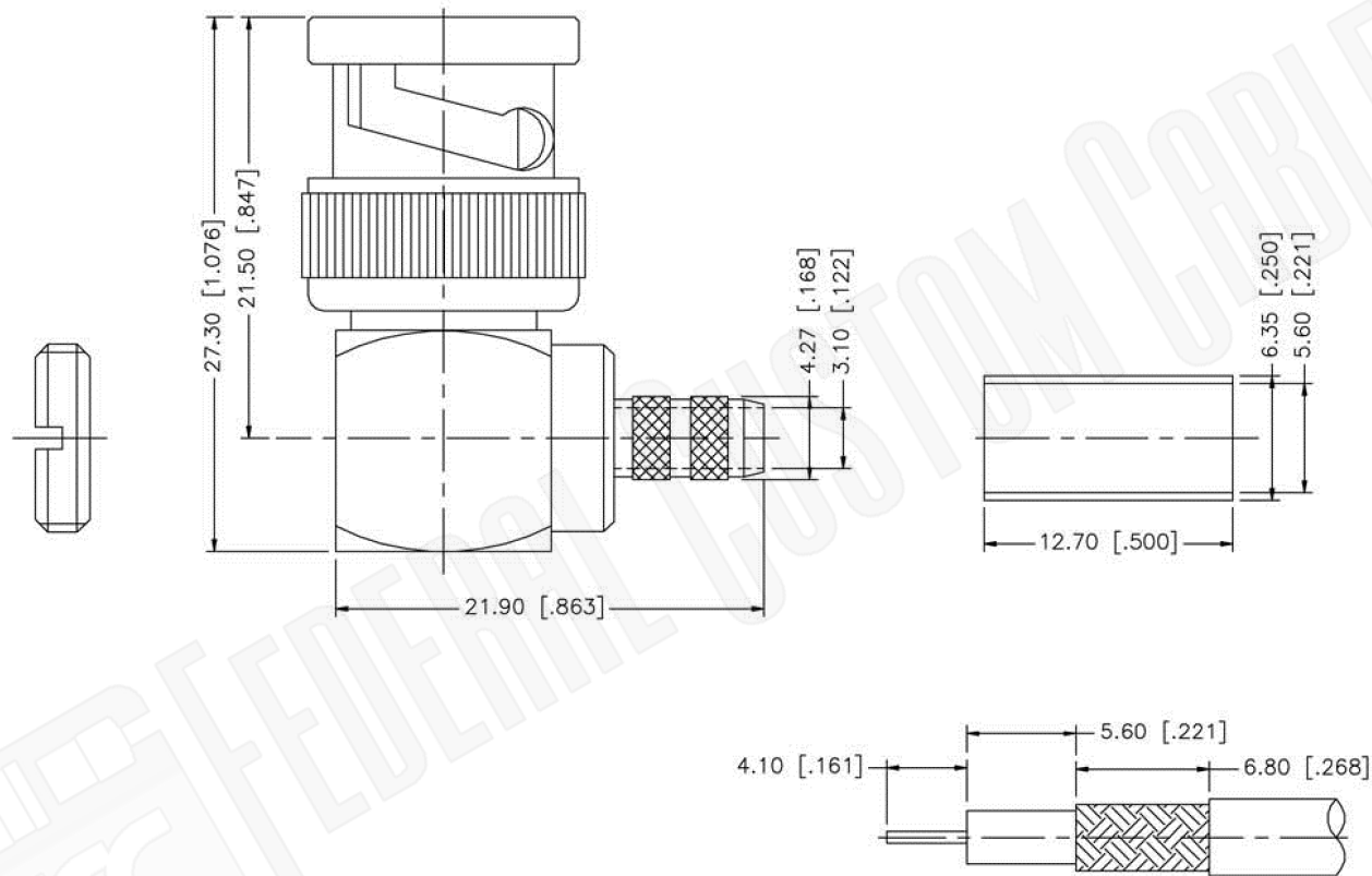
RECOMMENDED CABLE STRIPPING DIM'S
