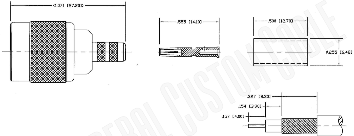
RECOMMENDED CABLE STRIPPING DIM'S
