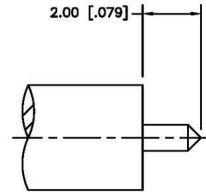
RECOMMENDED CABLE STRIPPING DIM'S
