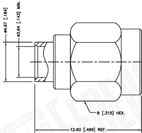
RECOMMENDED CABLE STRIPPING DIM'S
