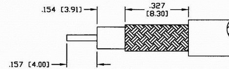
RECOMMENDED STRIPPING DIMENSIONS
